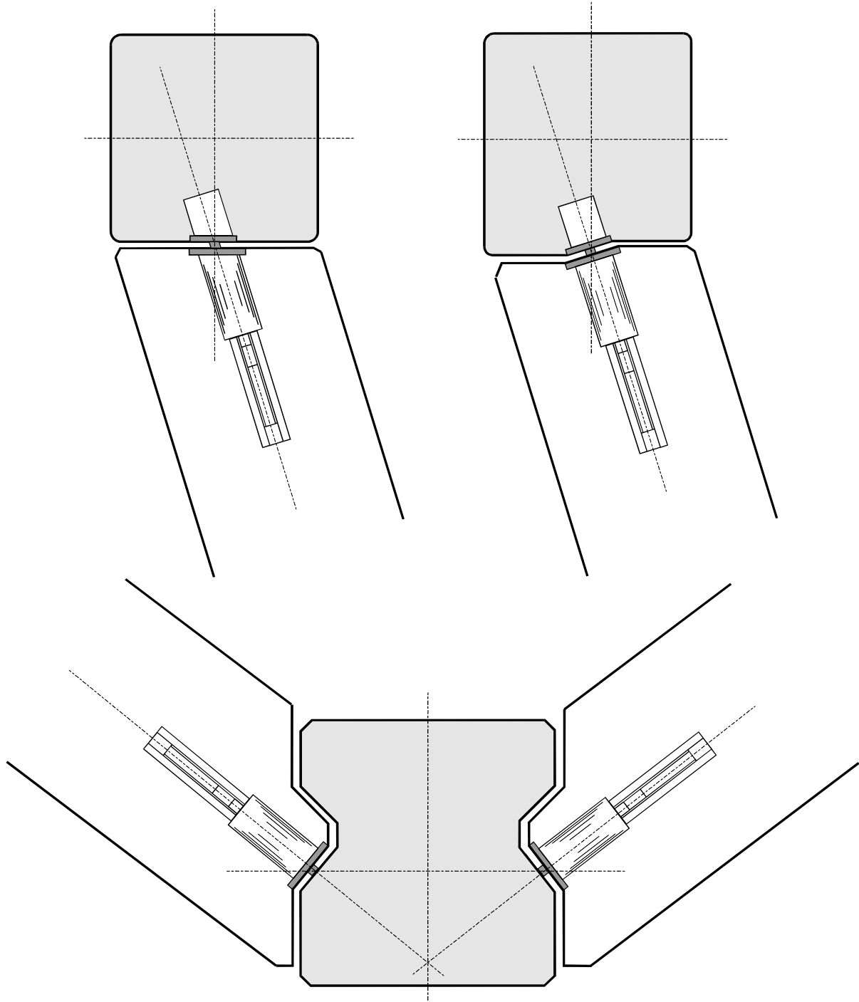
Figure shows a BSF unit
